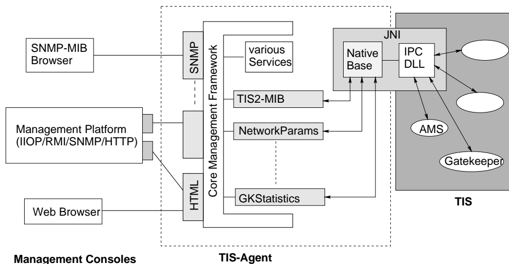
Figure 6: JDMK-based TIS Management: Architecture
