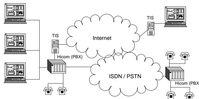
Figure 1: Siemens Telephony Internet Server: Architecture
