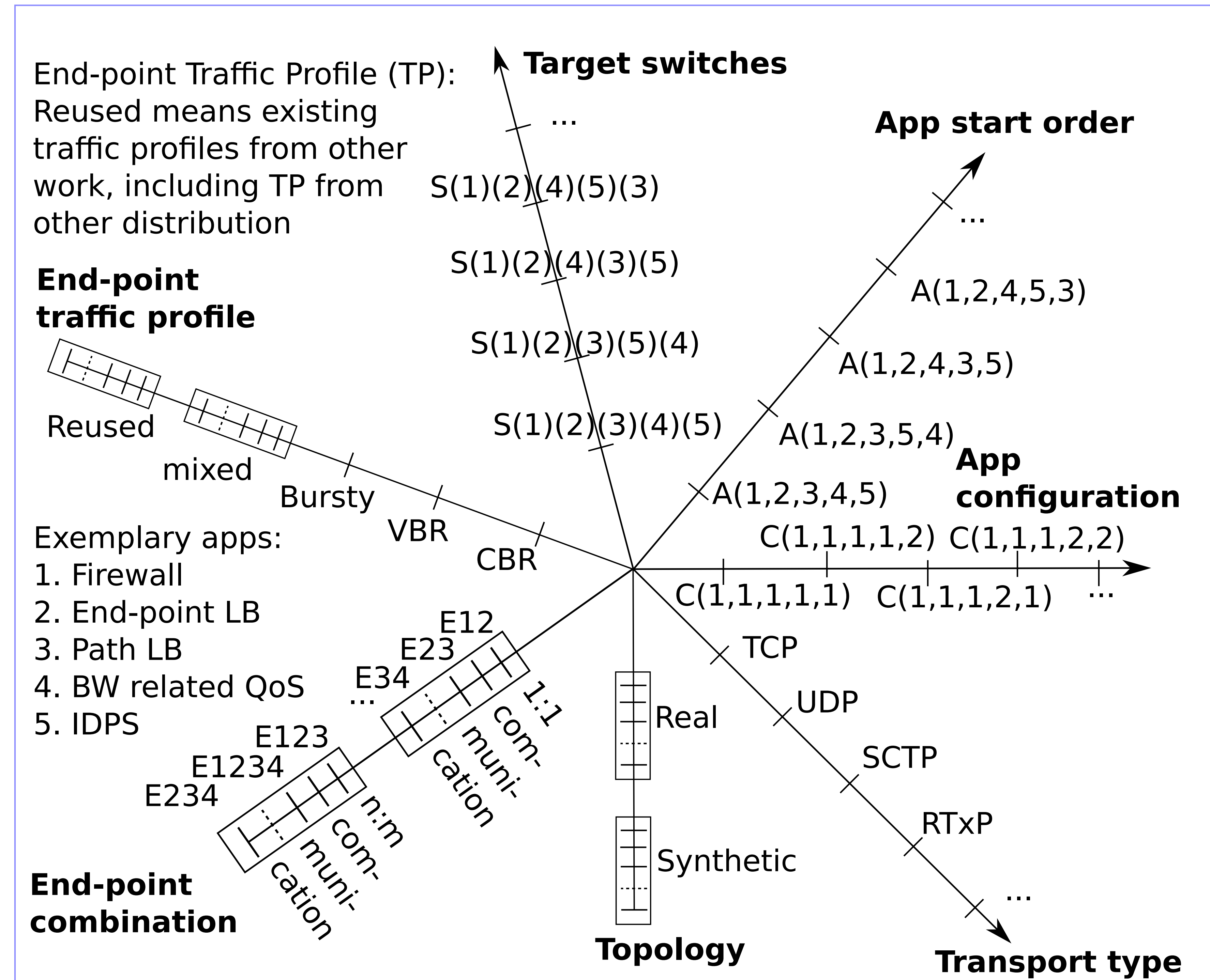
Parameter space for experimenting conflicts in SDN
